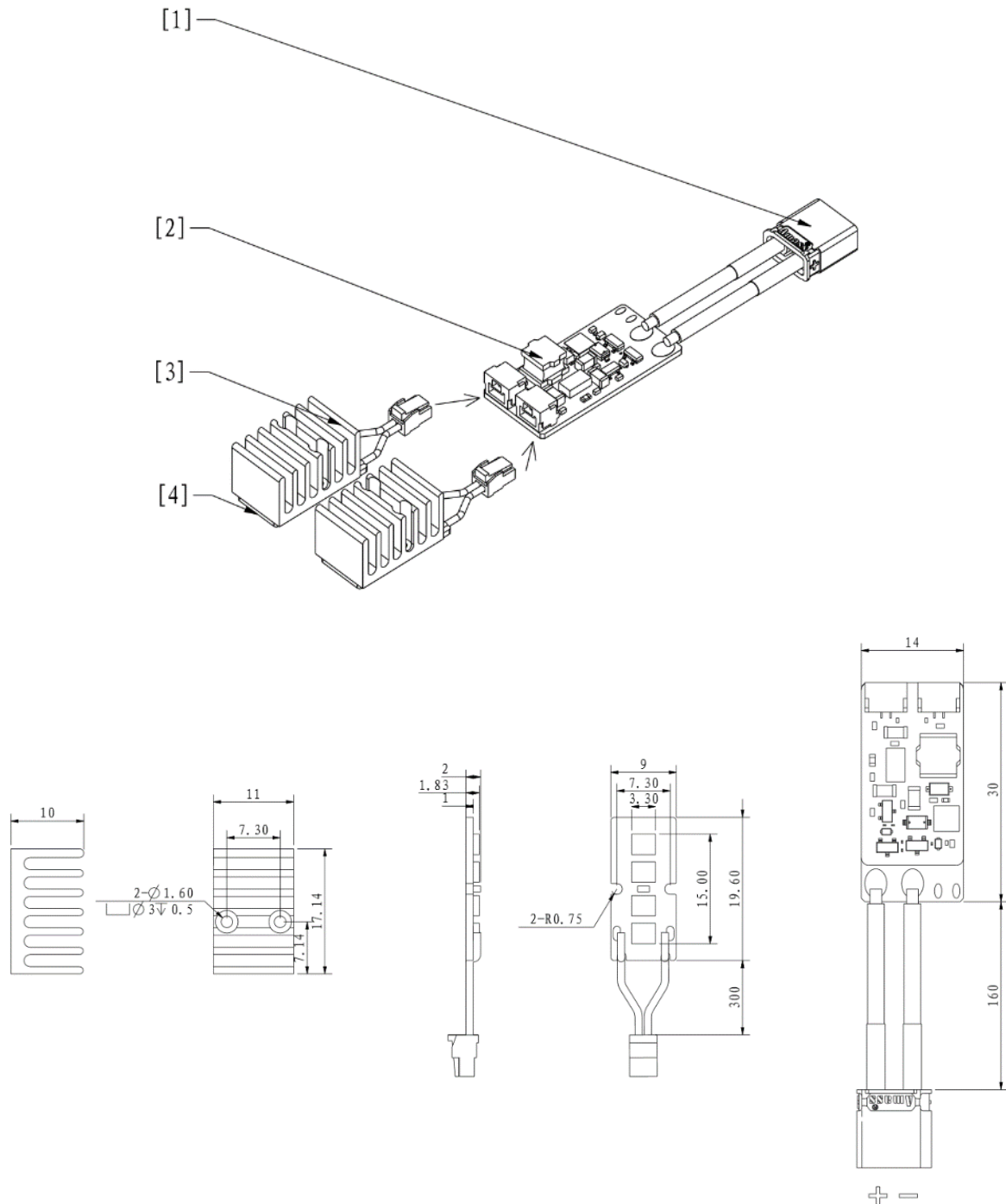
[1] XT30 port [2] LED actuator [3] Heat dissipation panel [4] UV light panel
