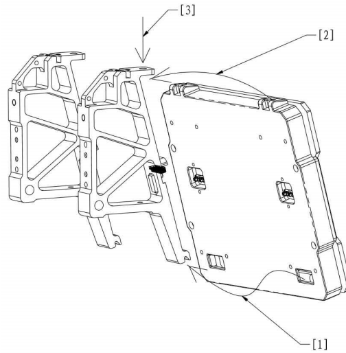
Figure 3-22 Armor Module Mounting Diagram
