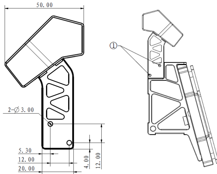
[1] Screw Hole Mounting Position
